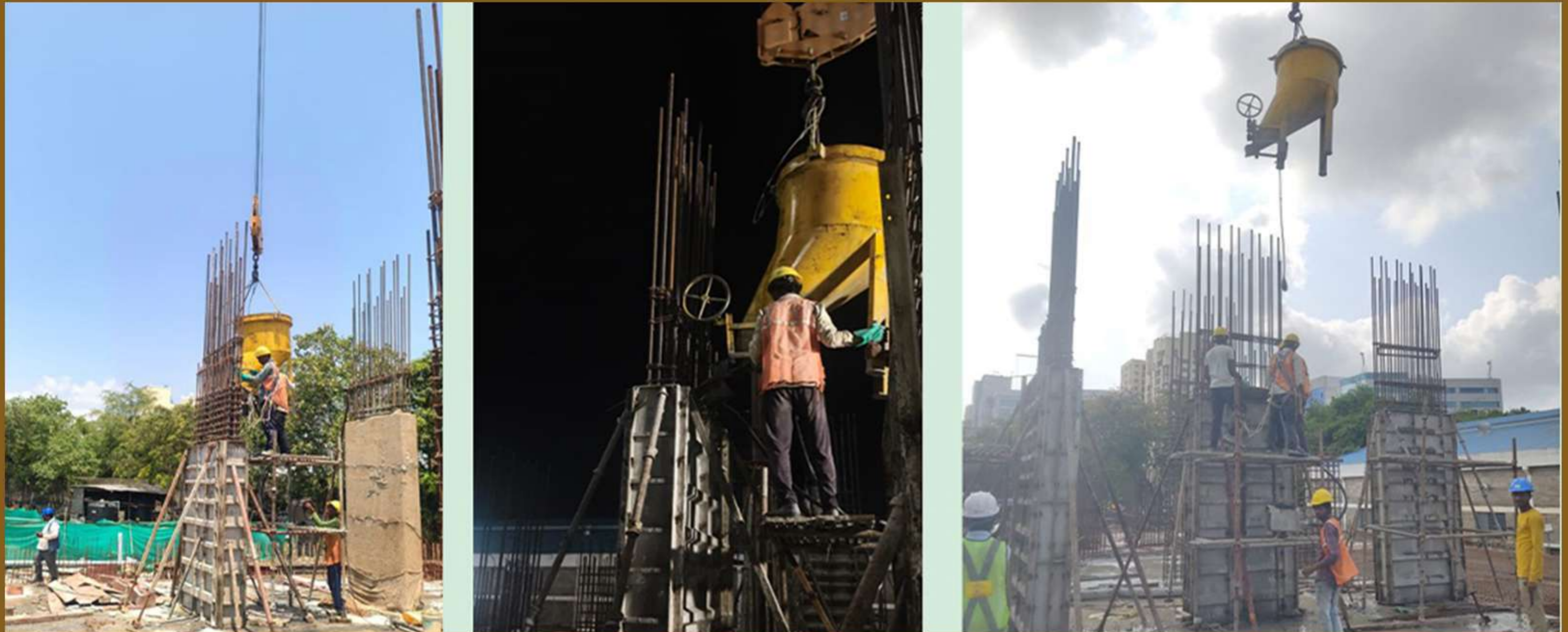
Block B Column Concrete Work In Stilt Floor
