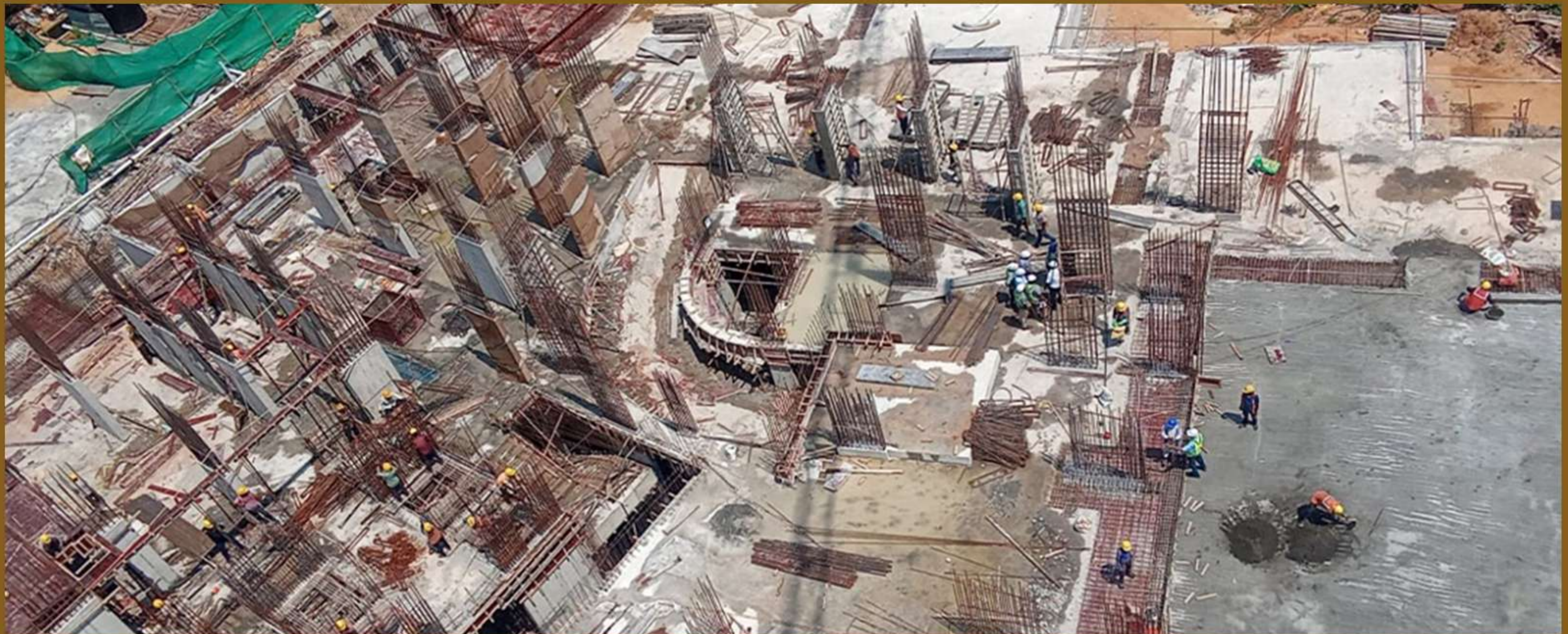
Block B Basement-1 Roof Concrete Work
