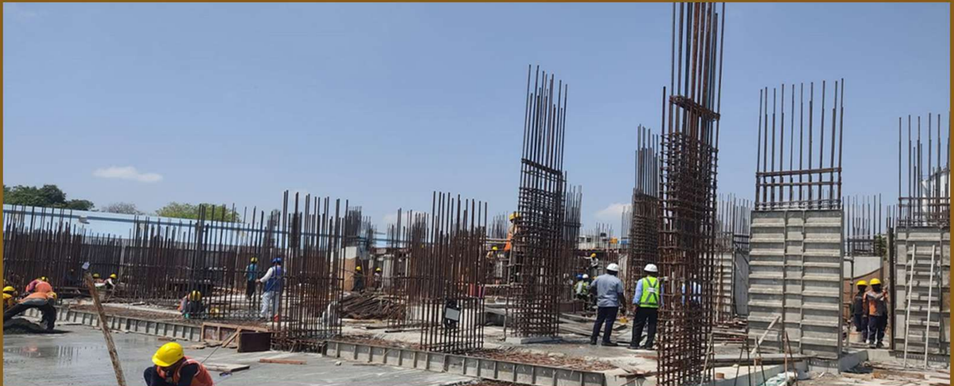
Block B Column Reinforcement Work In Stilt Floor
