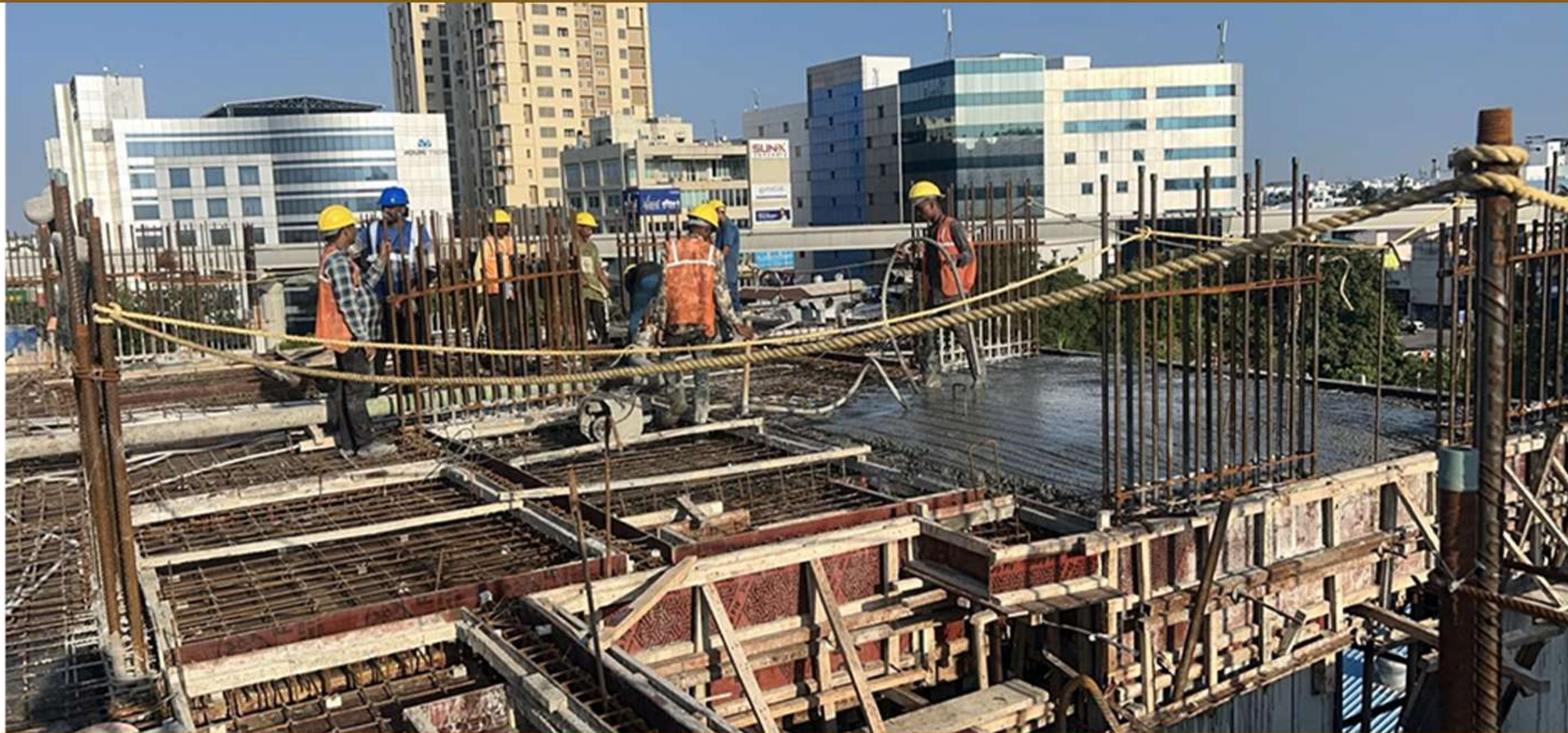
Block b – 4th Floor roof slab concrete work
