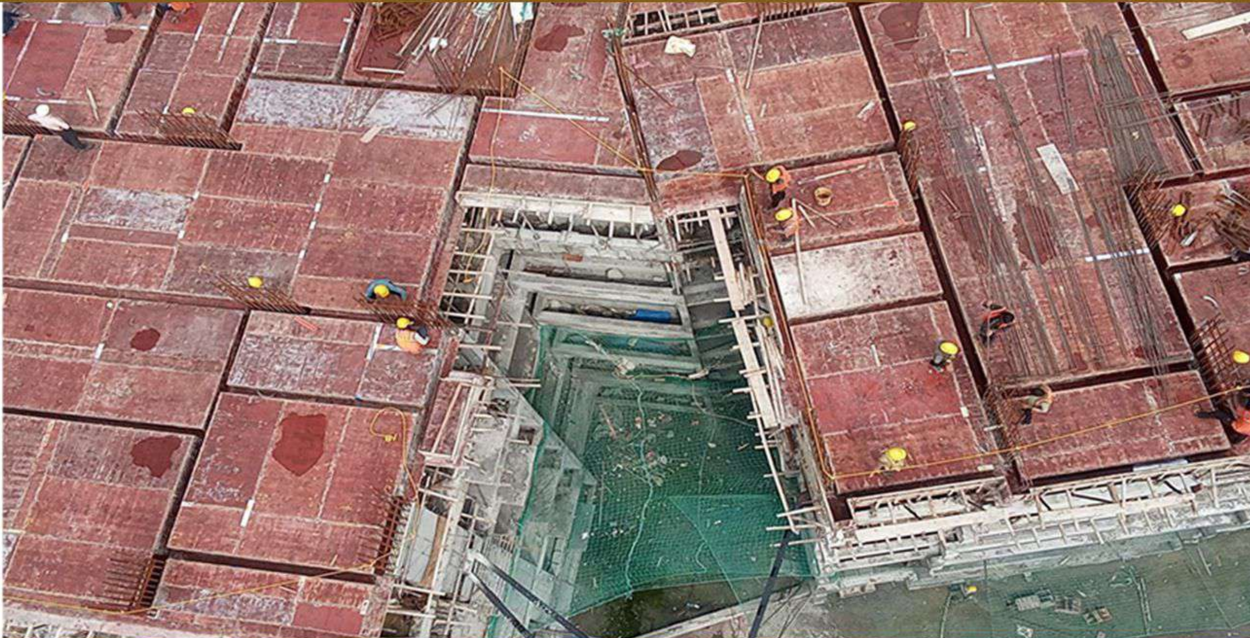
Block b – 6th floor roof slab Shuttering (Pour-2)
