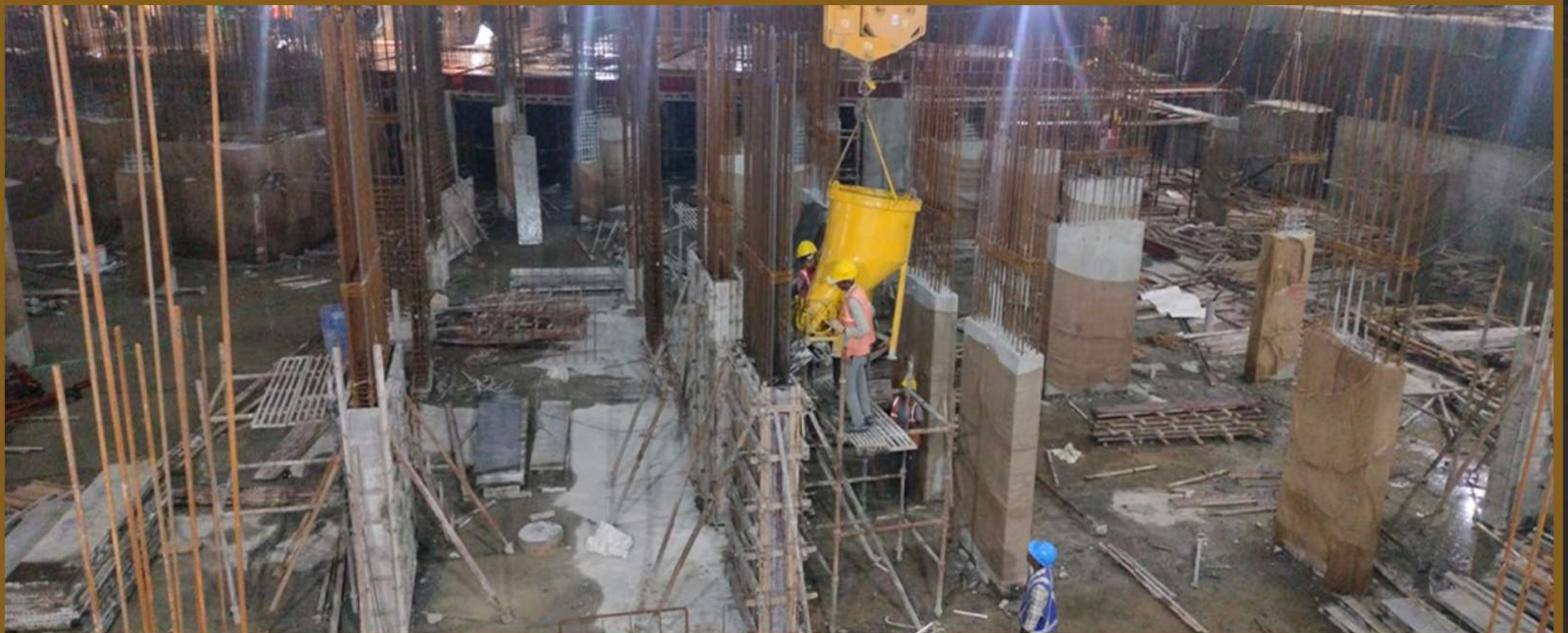
Block B column concrete work in basement-2
