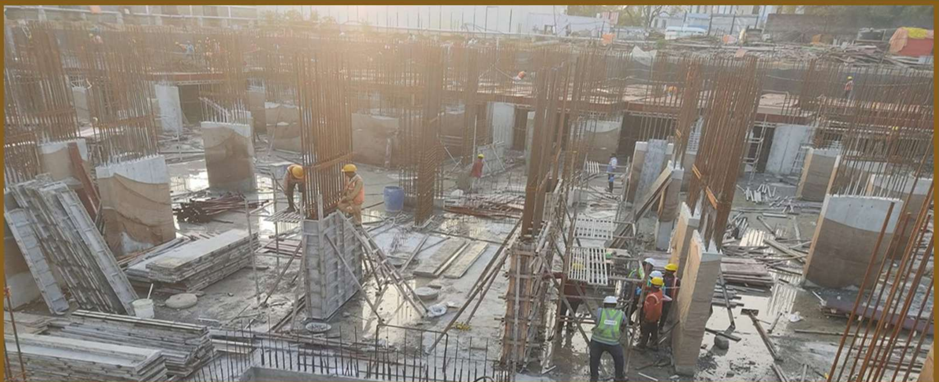
Block B column shuttering work in basement-2
